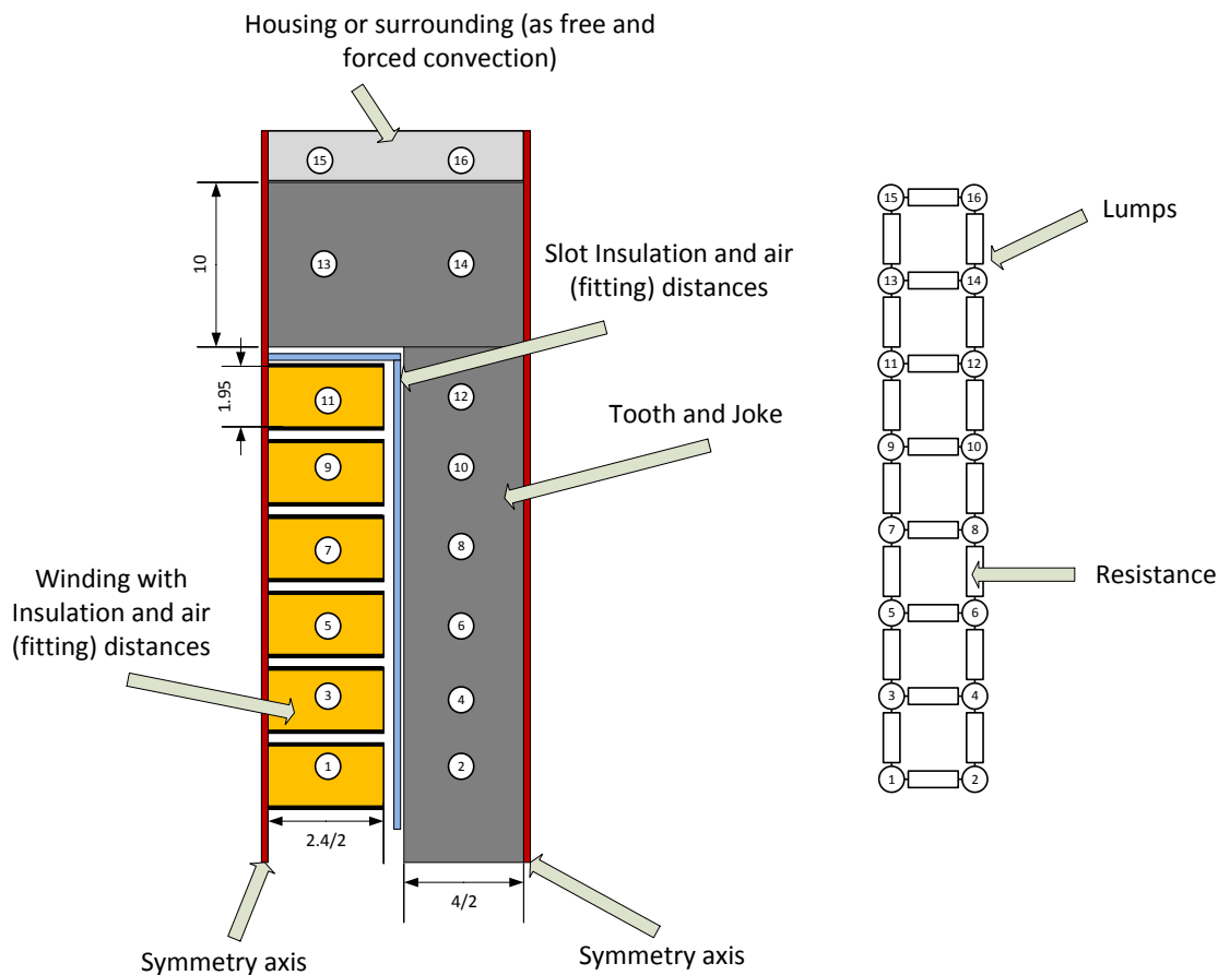
Figure 1: Lumped parameter model of a slot-tooth-symmetry unit of an electrical machine
